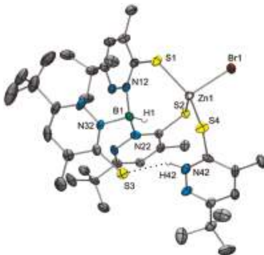
Figure 6. Molecular structure of [\text{Tn}^{\text{Me,tBu}}]\text{Zn}(\text{HPn}^{\text{Me,tBu}})\text{Br} (3). Hydrogen atoms, except for those on B1 and N42, as well as solvent molecules are omitted for clarity. Hydrogen bonding is depicted in dashed lines.
