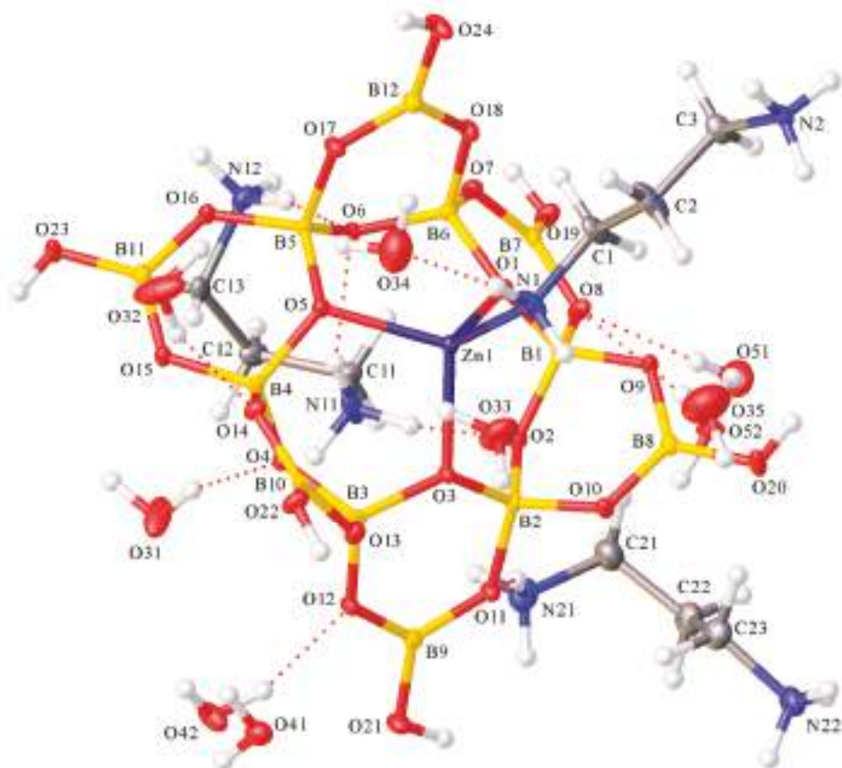
Figure 5. Diagram of (1,3\text{-pn})_3[\kappa^1N\text{-H}_3\text{N}(\text{CH}_2)_3\text{NH}_2]\text{Zn}[\kappa^3\text{O-B}_{12}\text{O}_{18}(\text{OH})_6]_2 \cdot 14\text{H}_2\text{O} (1,3-pn = 1,3-diaminopropane) ( 3 ) showing atomic labelling.
