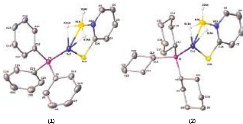
Figure 3. Molecular structures of [Cu( \kappa^3 -S,S,H,H-H 3 B(mp))](PR 3 ) (R = Ph, 1 ; Cy, 2 ). Thermal ellipsoids drawn at 50% level. Hydrogen atoms, with the exception of those attached to the boron centers, have been omitted for clarity. Both structures contain disorder in the position of the [H 3 B(mp)] − ligand. Only the major component is shown (see text for details).
