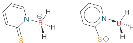
Figure 4. Two bonding descriptions for the [H 3 B(mp)] − .
