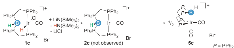
Figure 6. Reactivity of 1c towards base.
