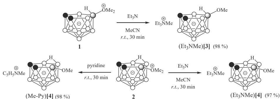
Scheme 2. Demethylation of dimethyloxonium derivatives of nido -carborane.
